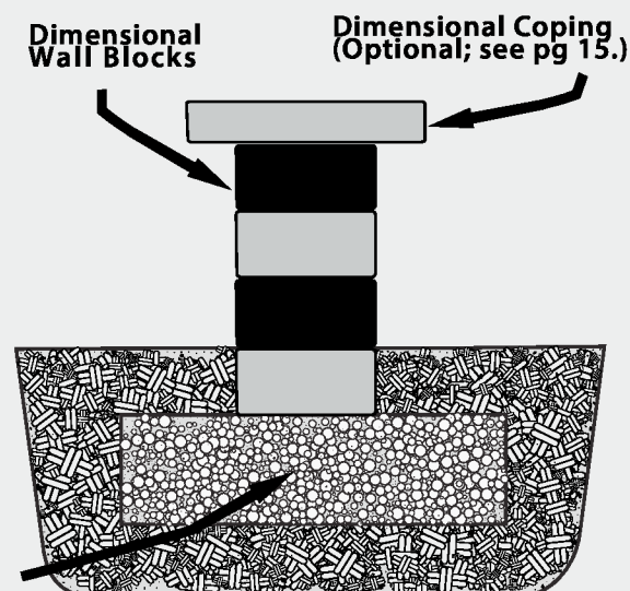
FREE STANDING WALL
