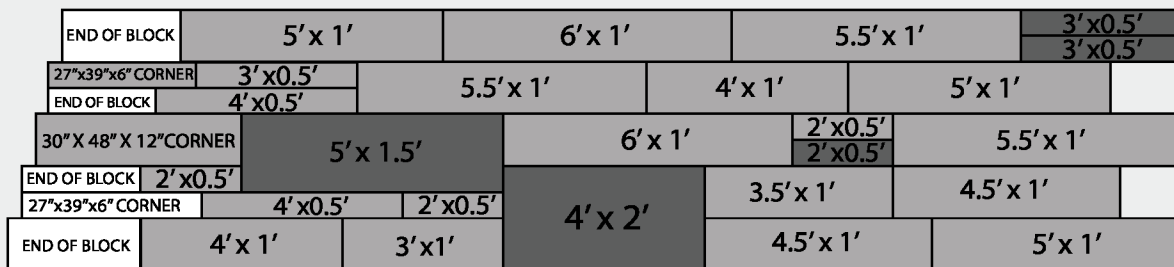
90° WALL CORNER
