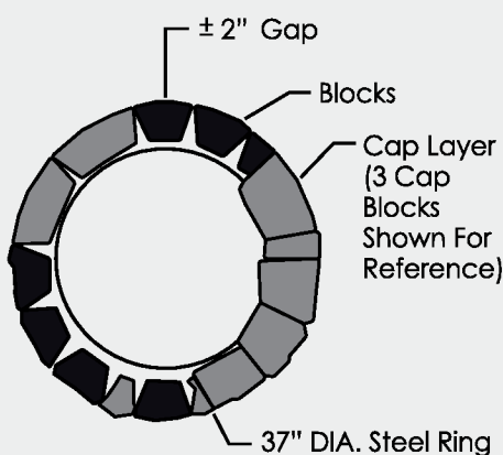
Round Fire Pit Pallet: 1,320 lbs
