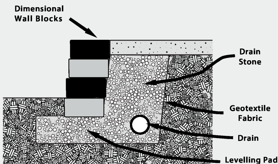
RETAINING WALL
