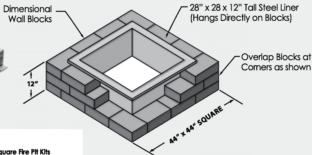
Square Fire Pit Pallet: 1,130 lbs
