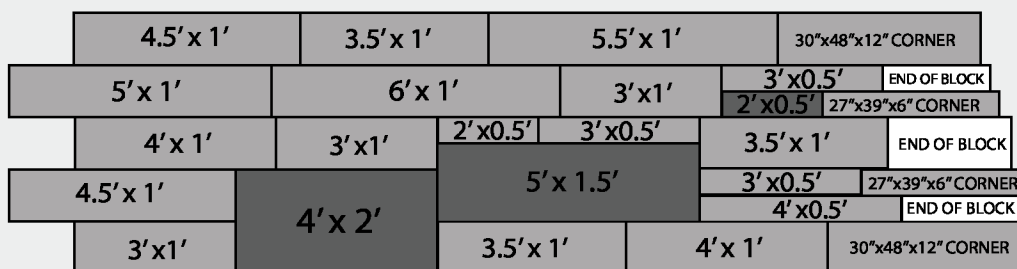
90° WALL CORNER
