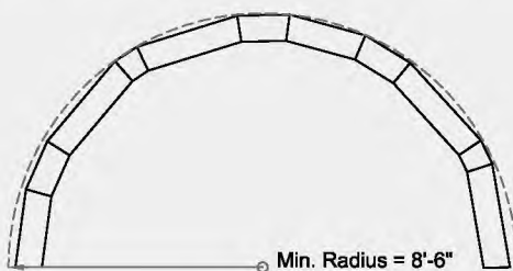
CONVEX RADIUS
