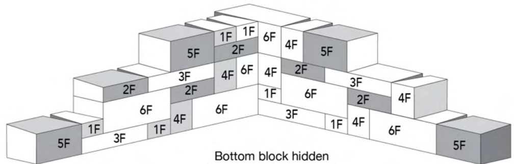
INSIDE CORNER
